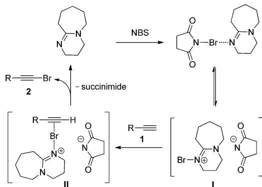
Scheme 5 Possible mechanism.
